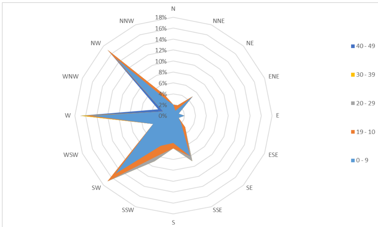
Figure 2.1 Distribution of 9AM wind speed and direction data during the reporting period
